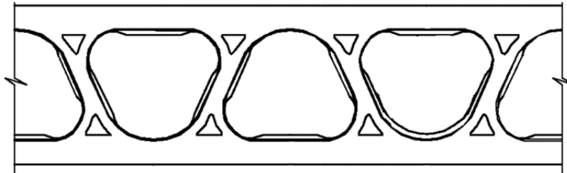
FIGURE 1—JOISTRITE® HOLES
